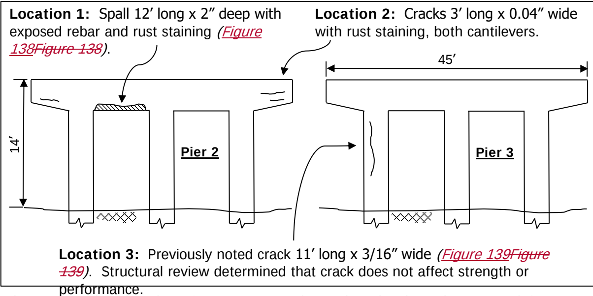
Figure 137. Elevation view of two concrete column piers showing substructure defect locations.
