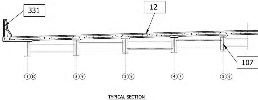
Figure 180. Typical bridge superstructure cross-section view from construction plans for a steel multi-beam bridge. (Source: Alabama DOT)
